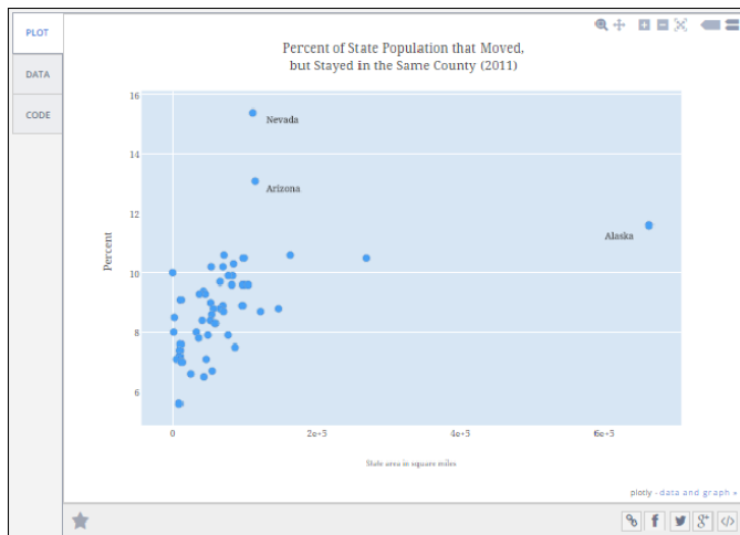
Figure 11-4: A scatter chart on Plotly.
